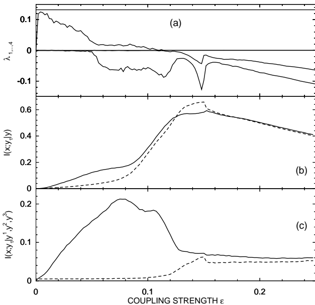
FIG. 4: (a) The two largest Lyapunov exponents of the drive \{X\} (constant lines) and the response \{Y\} (decreasing lines), (b) averaged conditional mutual information I(x; y_\tau | y) (solid line) and I(y; x_\tau | x) (dashed line), and (c) averaged CMI I(x; y_\tau | \vec{Y}) (solid line) and I(y; x_\tau | \vec{X}) (dashed line), where the vectors \vec{X} and \vec{Y} are the original components of the integrated systems, for the unidirectionally coupled Rössler systems (5),(6), as functions of the coupling strength \epsilon . The Lyapunov exponents are measured in nats per a time unit; the conditional mutual information in all figures is measured in units of nats.
