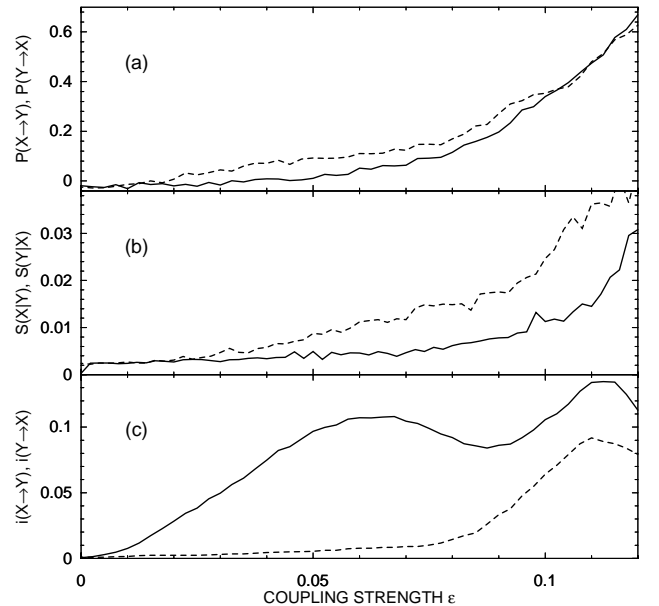
FIG. 3: (a) Cross-predictability P(X \rightarrow Y) (solid line) and P(Y \rightarrow X) (dashed line), (b) relative average distance of the mutual nearest neighbours S^{(k)}(\mathbf{Y}|\mathbf{X}) (solid line) and S^{(k)}(\mathbf{X}|\mathbf{Y}) (dashed line), and (c) coarse-grained transinformation rate i(X \rightarrow Y) (solid line) and i(Y \rightarrow X) (dashed line) for the unidirectionally coupled Rössler systems (5),(6), as functions of the coupling strength \epsilon .
