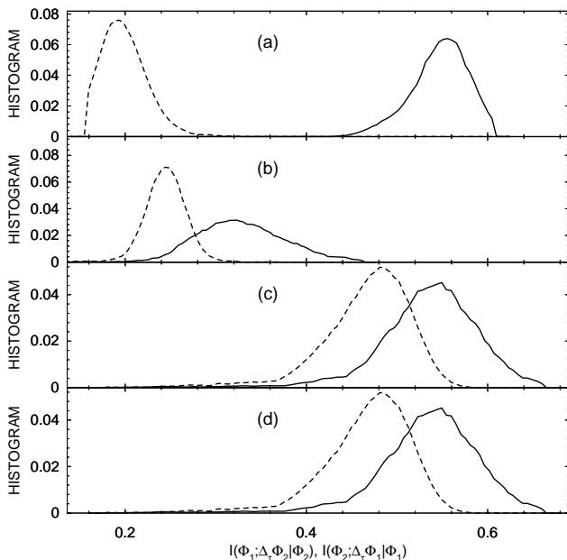
FIG. 6: Histograms of estimates of I(\phi_1; \Delta_\tau \phi_2 | \phi_2) (solid lines) and I(\phi_2; \Delta_\tau \phi_1 | \phi_1) (dashed lines) from 1000 realizations of (a) the unidirectionally coupled Rössler systems (5),(6), the coupling strength \epsilon = 0.05 and the number of samples N = 1024 , (b) FFT surrogate data for the data used in (a), N = 1024 ; (c) the same as in (a), but the number of samples N = 512 , and (d) FFT surrogate data for the data used in (c), N = 512 .
