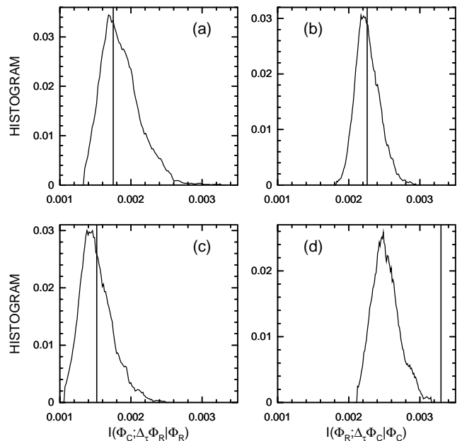
FIG. 11: Tests of causal influences of cardiac oscillations on respiratory oscillations measured by I(\phi_C; \Delta_\tau \phi_R | \phi_R) (a, c) and of the influence of the respiratory rhythm on the cardiac oscillations given by I(\phi_R; \Delta_\tau \phi_C | \phi_C) (b, d). Values from the tested data are marked by the vertical lines, the surrogate ranges are illustrated by the histograms obtained from 2500 surrogate realizations. (a,b) The test of bias using data from two animals; (c,d) a real test for one of the animals.
