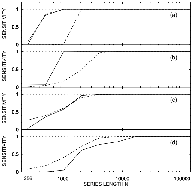
FIG. 9: (a) Sensitivity as function of time series length N for the tests using the coupled Rössler systems (5),(6) with the frequency ratio 1:1 (dash-and-dotted line), 5:1 (solid line) and 1:5 (dashed line) for a_1 = a_2 = 0.15 . The Hilbert phases were used. (b) Sensitivity of the tests for the coupled Rössler systems (5),(6) with the frequency ratio 5:1 (solid line) and 1:5 (dashed line) for a_1 = a_2 = 0.15 , as the function of the series length N . The marked events phases were used. (c) Sensitivity as function of time series length N for the tests using the coupled Rössler systems (5),(6) with the frequency ratio 5:1, a_1 = 0.72 , a_2 = 0.15 (solid line) and 1:5, a_1 = 0.15 , a_2 = 0.72 (dashed line). The Hilbert phases were used. (d) The same as in (c), but the marked events phases were used.
