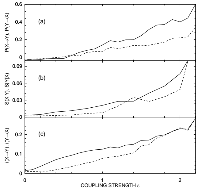
FIG. 1: (a) Cross-predictability P(X \rightarrow Y) (solid line) and P(Y \rightarrow X) (dashed line), (b) relative average distance of the mutual nearest neighbours S^{(k)}(\mathbf{Y}|\mathbf{X}) (solid line) and S^{(k)}(\mathbf{X}|\mathbf{Y}) (dashed line), and (c) coarse-grained transinformation rate i(X \rightarrow Y) (solid line) and i(Y \rightarrow X) (dashed line) for the Rössler system (1) driving the Lorenz system (2), as functions of the coupling strength \epsilon .
