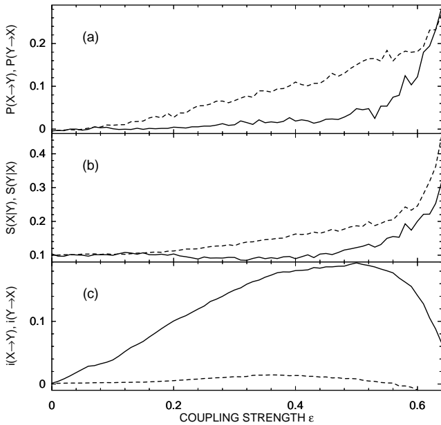
FIG. 2: (a) Cross-predictability P(X \rightarrow Y) (solid line) and P(Y \rightarrow X) (dashed line), (b) relative average distance of the mutual nearest neighbours S^{(k)}(\mathbf{Y}|\mathbf{X}) (solid line) and S^{(k)}(\mathbf{X}|\mathbf{Y}) (dashed line), and (c) coarse-grained transinformation rate i(X \rightarrow Y) (solid line) and i(Y \rightarrow X) (dashed line) for the unidirectionally coupled Henon system (3),(4), as functions of the coupling strength \epsilon .
