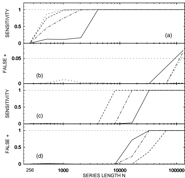
FIG. 10: Sensitivity (a,c) and the rate of false positives (b,d) as functions of time series length N for the tests using the coupled Rössler systems (5),(6) with the frequency ratio 1:1 for different amounts of noise in the data. The portions of noise are in (a,b) 0% (dotted line), 10% (dashed line), 20% (dash-and-dotted line) and 30% (solid line); in (c,d) 50% (dashed line), 70% (dash-and-dotted line) and 100% (solid line).
