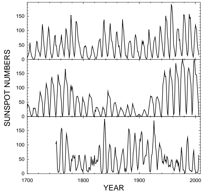
FIG. 15: The yearly sunspot numbers 1700–2006 (top panel). A 307-sample realization of the Barnes model (middle panel). A realization of the IAFT surrogate data of a 256-sample subset of the sunspot numbers (bottom panel).
