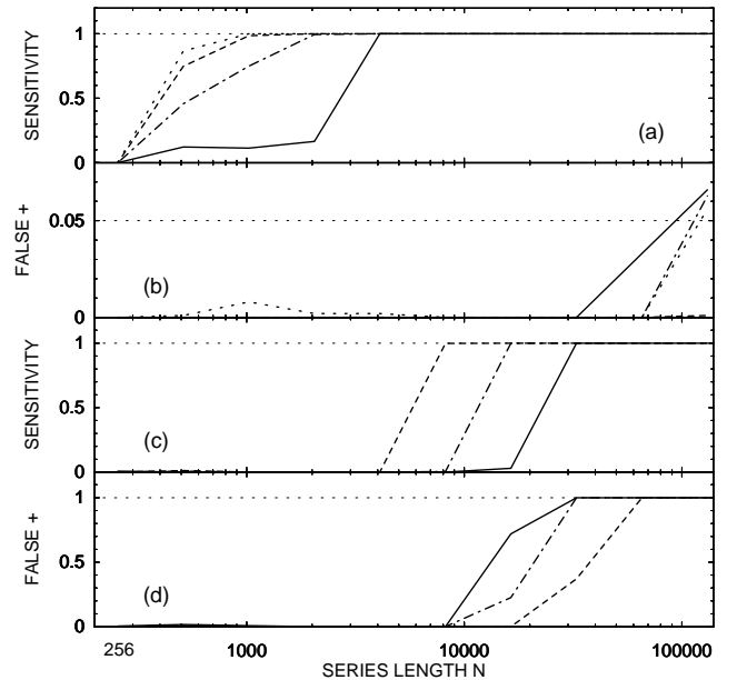
FIG. 28: Sensitivity (a,c) and the rate of false positives (b,d) as functions of time series length N for the tests using the coupled Rössler systems (43),(44) with the frequency ratio 1:1 for different amounts of noise in the data. The portions of noise are in (a,b) 0% (dotted line), 10% (dashed line), 20% (dash-and-dotted line) and 30% (solid line); in (c,d) 50% (dashed line), 70% (dash-and-dotted line) and 100% (solid line).
