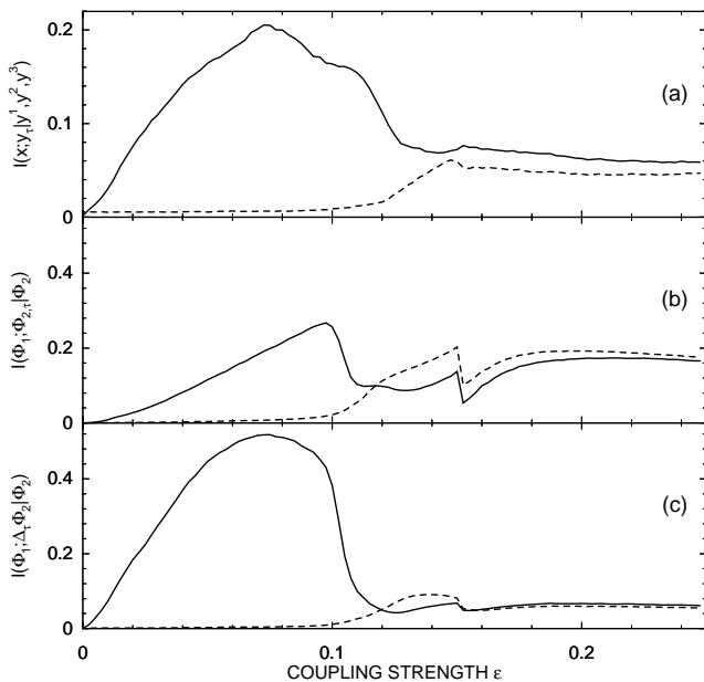
FIG. 26: (a) Averaged conditional mutual information I(x; y | \vec{Y}) (solid line) and I(y; x | \vec{X}) (dashed line), using the time-delay embedding vectors \vec{X} = [x_1(t), x_1(t-\eta), x_1(t-2\eta)] and analogously for \vec{Y} , (b) averaged CMI I(\phi_1(t); \phi_2(t + \tau) | \phi_2(t)) (solid line) and I(\phi_2(t); \phi_1(t + \tau) | \phi_1(t)) (dashed line), and (c) averaged CMI I(\phi_1; \Delta_\tau \phi_2 | \phi_2) (solid line) and I(\phi_2; \Delta_\tau \phi_1 | \phi_1) (dashed line), for the unidirectionally coupled Rössler systems (43),(44), as functions of the coupling strength \epsilon .
