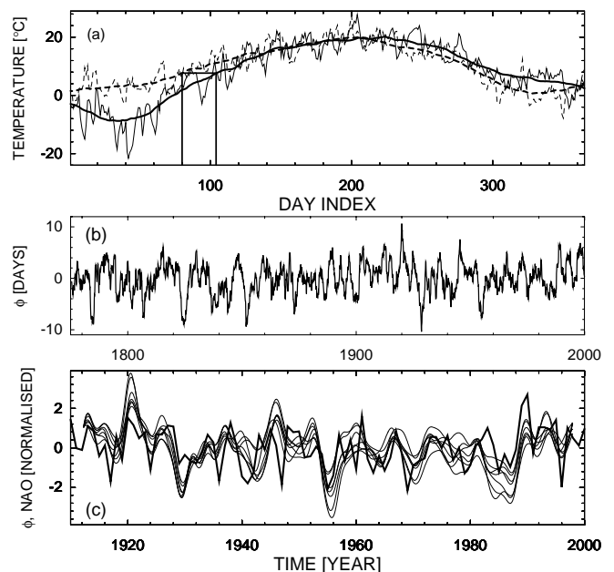
FIG. 14: (a) The daily mean near-surface air temperature in Prague in 1920 (dashed lines) and in 1929 (solid lines), raw data (thin lines) and smoothed data (thick lines). The solid straight lines show that the temperature of March 21, 1920 was reached with a delay of 24 days in 1929. (b) The phase \phi(t) of the annual temperature cycle obtained from the Prague record (1775 – 2001). (c) The phase \phi(t) of the annual temperature cycle obtained from seven European stations (thin smooth lines); and the North Atlantic Oscillation index averaged over the January-March period (thick line). All data are normalized to zero mean and unit variance.
