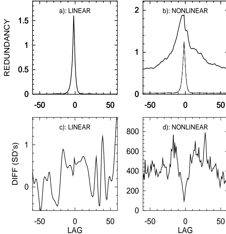
Figure 2: a): Linear redundancy L(x(t); y(t + \tau_1); z(t)) , b): nonlinear (general) redundancy R(x(t); y(t + \tau_1); z(t)) , for the chaotic three-dimensional Lorenz system ( thick line ) and for related isospectral surrogates ( thin line, coinciding in a, but different in b ); c): linear , and d): nonlinear statistics ; as functions of the time lag \tau_1 .
