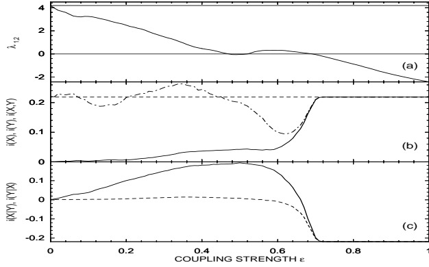
FIG. 1. (a) The largest Lyapunov exponents of the drive \{X\} (constant line) and the response \{Y\} (decreasing line), (b) the CIR i(X) of the drive (dashed line) and i(Y) of the response (dash-and-dotted line) and the mutual CIR i(X, Y) (full line), (c) the coarse-grained transinformation rates i(X|Y) (dashed line) and i(Y|X) (full line) for the unidirectionally coupled identical ( b_1 = b_2 = 0.3 ) Henon systems. The Lyapunov exponents are measured in nats per time unit, the CIR's in nats.
